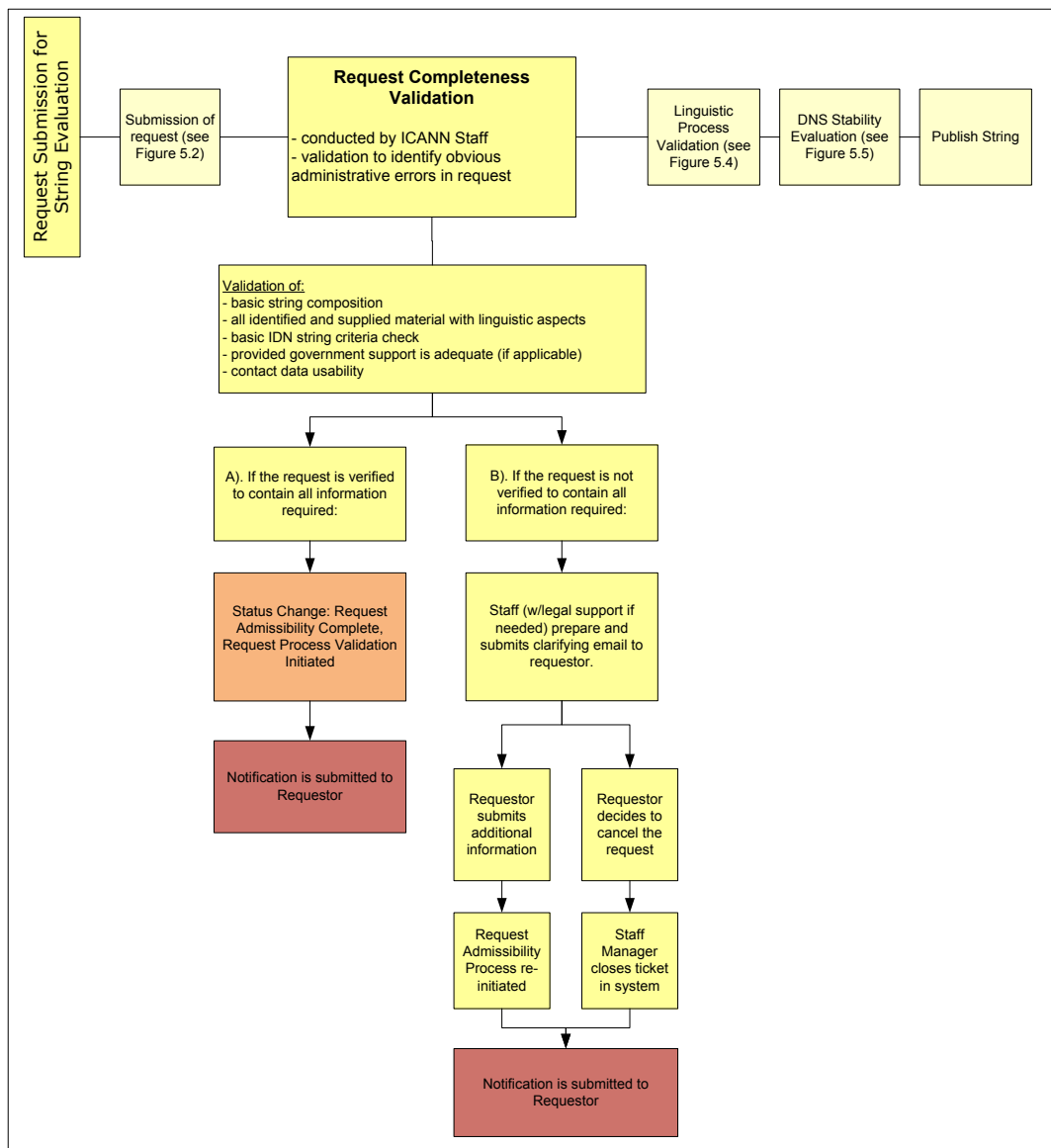
Figure 5.3: Stage 2: Request Completeness Validation.
