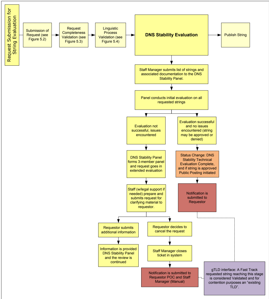
Figure 5.5: Stage 2: DNS Stability Evaluation.
